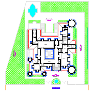
Third Floor Plan A = 286.99 m 2
