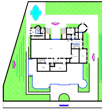
Lower Floor Plan A = 395.06 m 2
