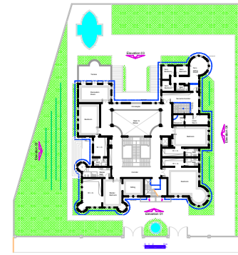
Second Floor Plan A = 479.38 m 2
