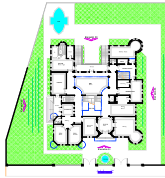
First Floor Plan A = 540.68 m 2
